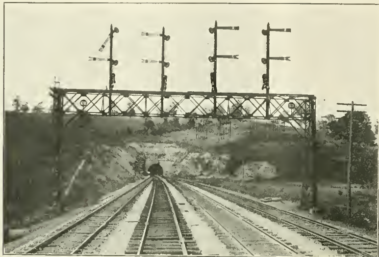
RADEBAUGH TUNNEL ON THE PENNSYLVANIA RAILROAD. Both Eastbound and Both Westbound Tracks Gauntleted.
